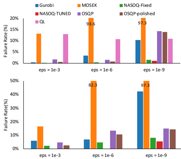
Fig. 3. Failure rate of NASOQ-Fixed, NASOQ-Tuned, OSQP, OSQP-Polished, Gurobi, QL, and MOSEK across different ranges of accuracy ( 10^{-3} , 10^{-6} , and 10^{-9} ) and for both small-scale (top) and large-scale (bottom) QP problems. NASOQ-tuned has the lowest failure rate compared to all other QP solvers for problems of different scales and for different requested accuracies.
